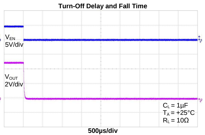
Figure 1. Voltage Waveforms
