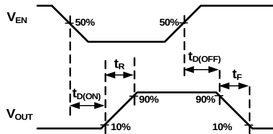
Figure 1. Voltage Waveforms
