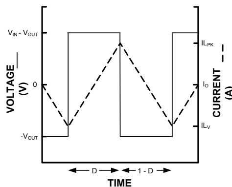
FIGURE 5. INDUCTOR WAVEFORM
