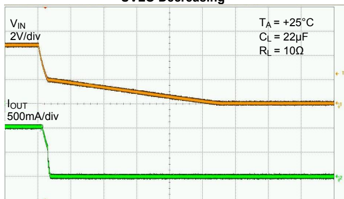
UVLO Decreasing
