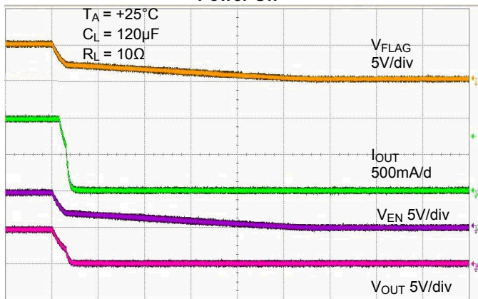
Power Off
