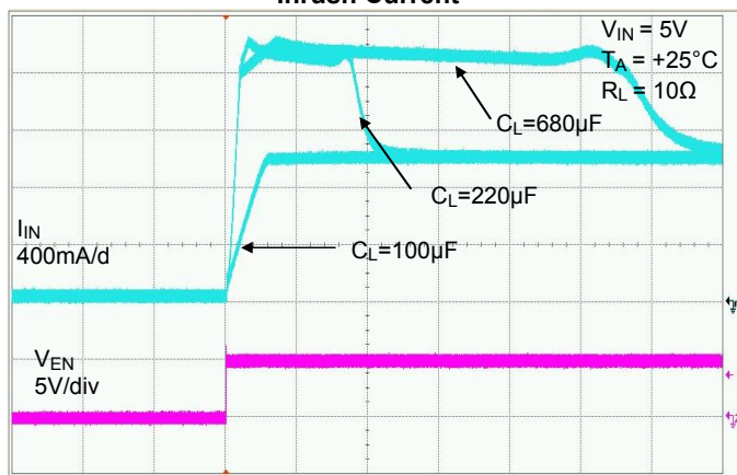
Inrush Current
