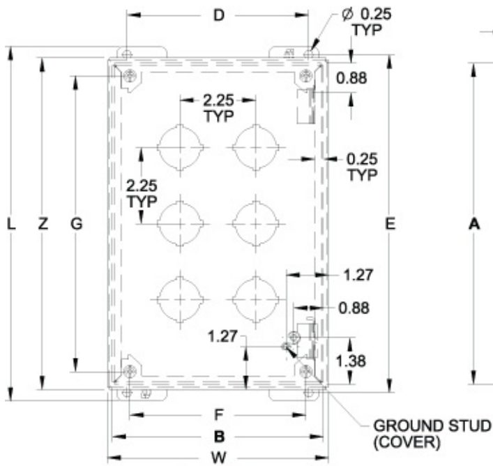
Front View Body Type F through S (Hinged)
