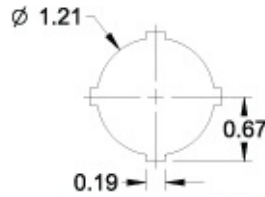
30.5mm Detail (1435 Series)
