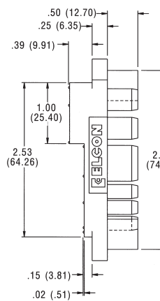
Float-Mount Part Number 6648167-1
