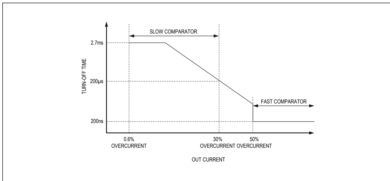
Figure 3. VariableSpeed/BiLevel Response
