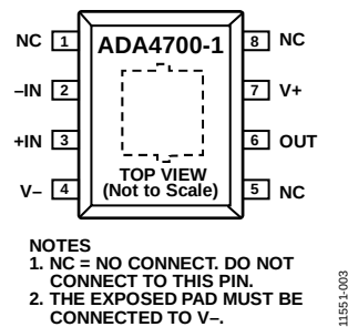
Figure 2. Pin Configuration
