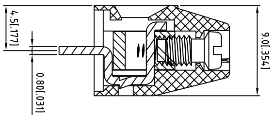
SECTION P-P
