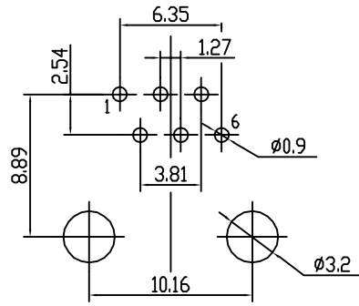
6P6C
