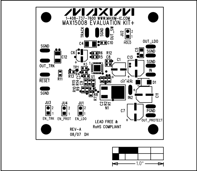
Figure 2. MAX15008 EV Kit Component Placement Guide—Component Side
