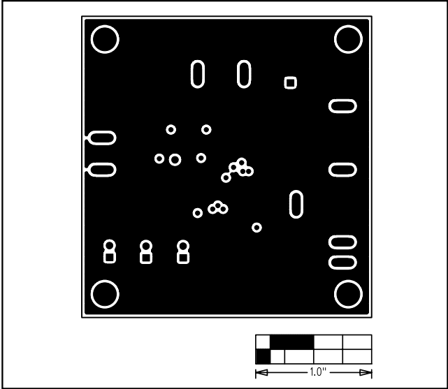
Figure 4. MAX15008 EV Kit PCB Layout—Ground Layer (Layer 2)
