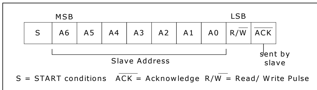
Figure 41. 7-Bit Address Format
