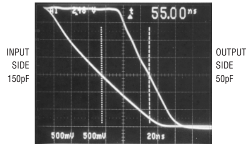
Figure 2. Input-Output Connection t_{PLH}
