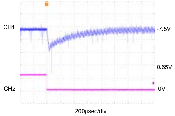
CH1:V OUT2 , AC-COUPLED ,20mV/div CH2:PWM 2 , 0.5V/div
