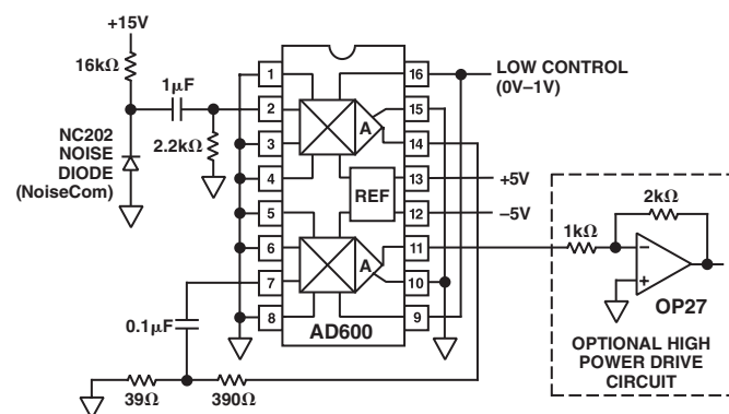
Figure 30. Noise Source (Dither Generator)
