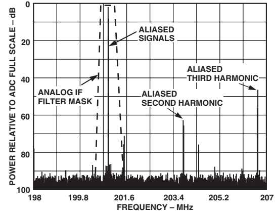
Figure 33. IF Sampling a 201 MHz Input
