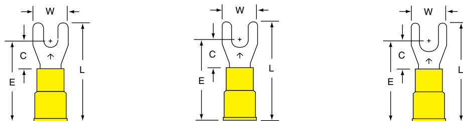
MV10-6F MV10-8F MV10-10F Stud Size 6 8 10 Wire Range 12-10 12-10 12-10
