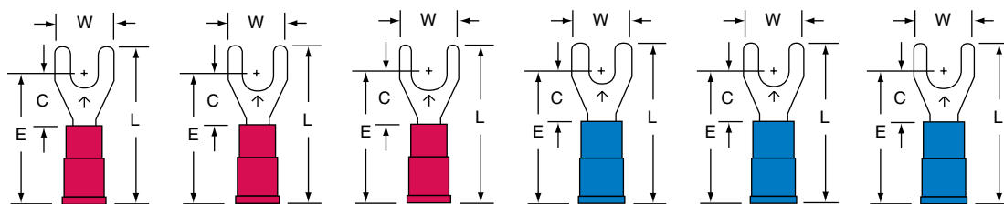
MV18-6F MV18-8F MV18-10F MV14-6F MV14-8F MV14-10F Stud Size 6 8 10 6 8 10 Wire Range 22-18 22-18 22-18 16-14 16-14 16-14
