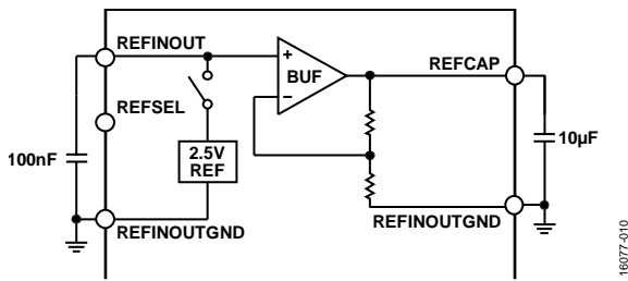
Figure 48. Reference Circuitry
