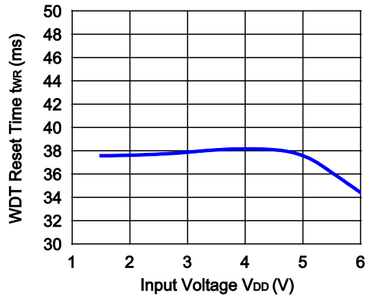
12) WDT Reset Timer vs. Input Voltage R510xx
