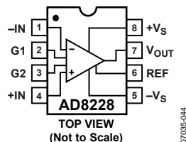
Figure 44. Pinout Diagram
