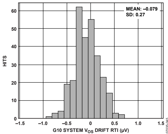
Figure 4. Typical Distribution of Input Offset Voltage Drift (G = 10)
