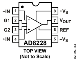
Figure 44. Pinout Diagram
