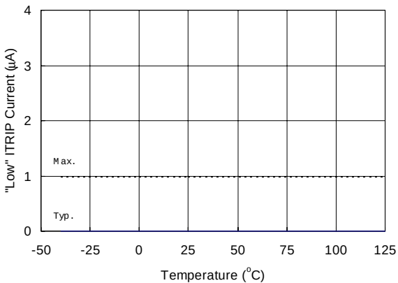
Figure 25A. "Low" ITRIP Current vs. Temperature
