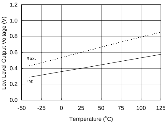
Figure 17A. Low Level Output vs. Temperature
