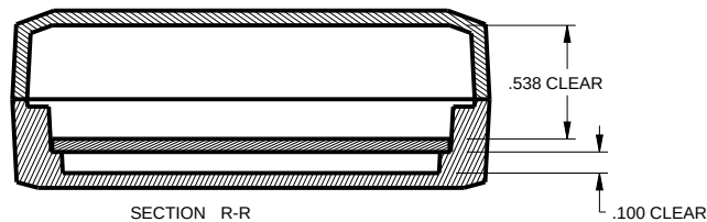
SECTION R-R
