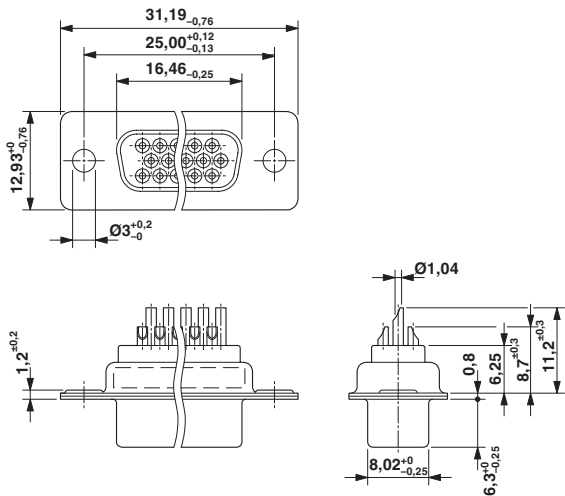
Dimensioned drawing
