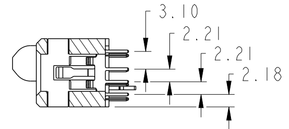
SECTION Z-Z
