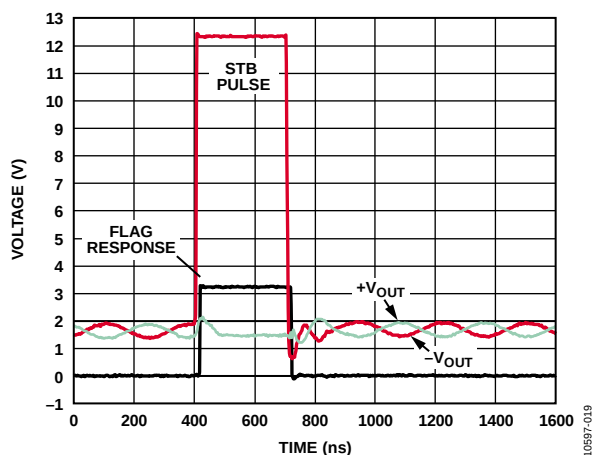
Figure 16. STB Output Flag Response Time
