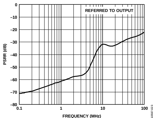
Figure 20. Power Supply Rejection Ratio (PSRR) vs. Frequency
