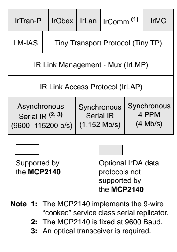
FIGURE B-2: IRDA DATA - PROTOCOL STACKS
