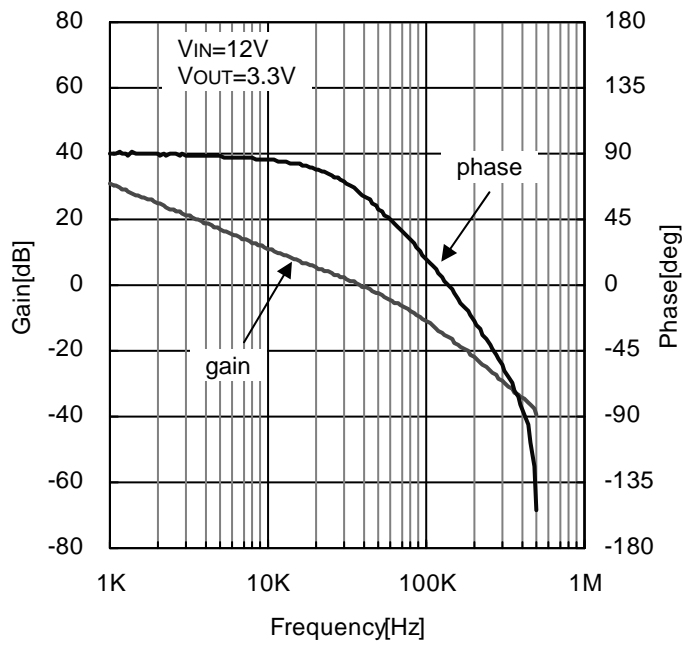
Figure 39. Loop Response IOUT=1A (VIN=12V, VOUT=3.3V, COUT=Ceramic10μF × 3)
