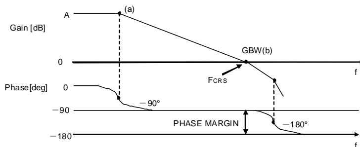
Figure 53. Bode plot
