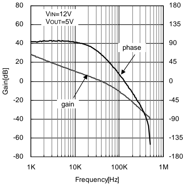
Figure 38. Loop Response IOUT=1A (VIN=12V, VOUT=5V, COUT=Ceramic10μF × 3)
