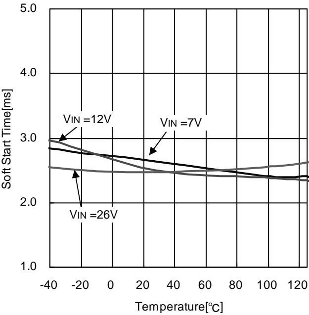
Figure 17. Soft Start Time - Temperature
