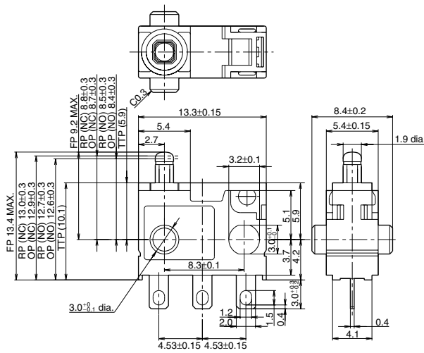
External dimensions
