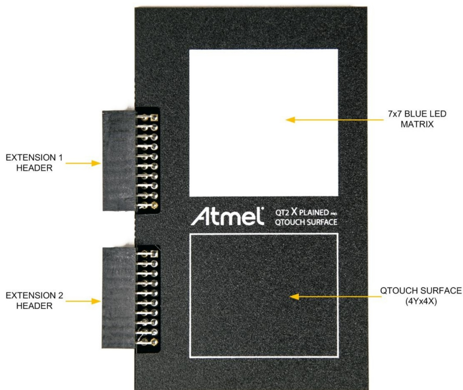
Figure 1-1. QT2 Xplained Pro Extension Board
