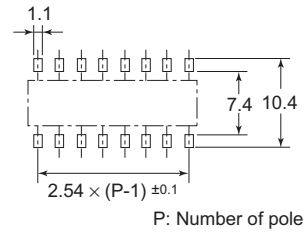
Dimensions of PCB Pad (Reference) (Top View)
