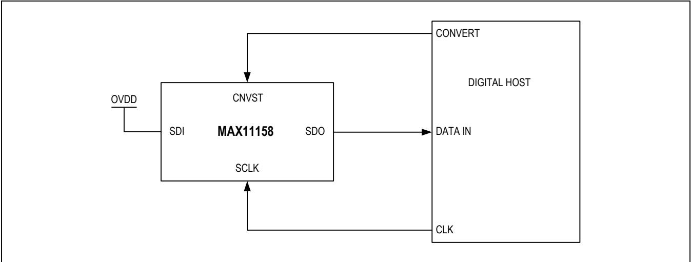
Figure 5. \overline{CS} Mode 3-Wire, No-Busy Indicator Connection Diagram ( \overline{SDI} High)
