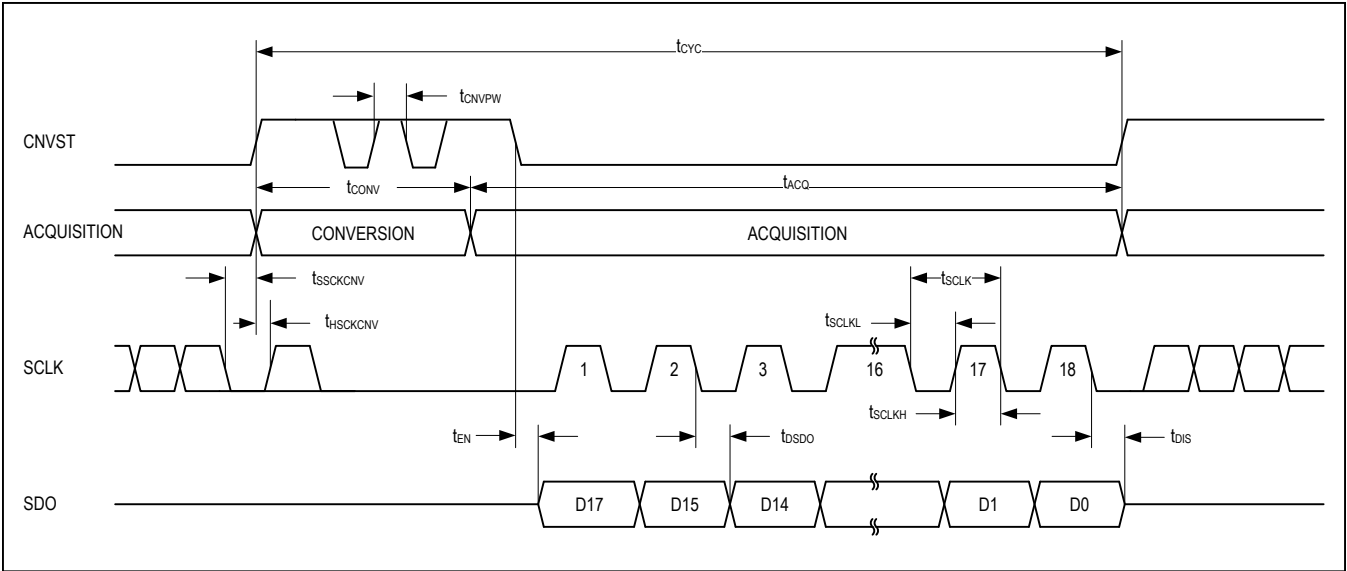
Figure 6. \overline{CS} Mode 3-Wire, No-Busy Indicator Serial Interface Timing ( \overline{SDI} High)
