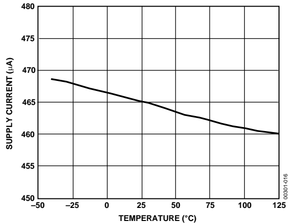
Figure 16. OP282 Supply Current vs. Temperature
