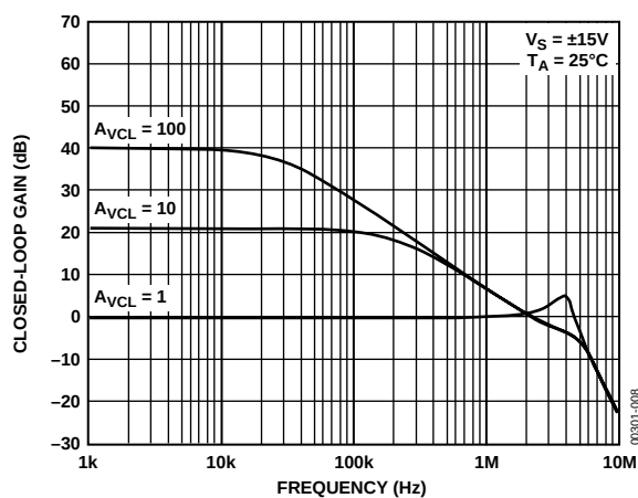
Figure 8. OP282 Closed-Loop Gain vs. Frequency
