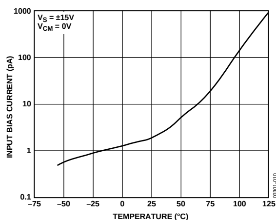
Figure 10. OP282 Input Bias Current vs. Temperature
