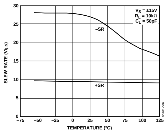
Figure 9. OP282 Slew Rate vs. Temperature
