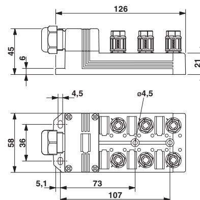
Dimensioned drawing
