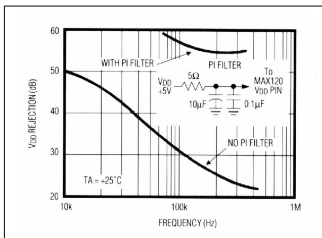
Figure 16. V_{DD} Power-Supply Rejection vs. Frequency
