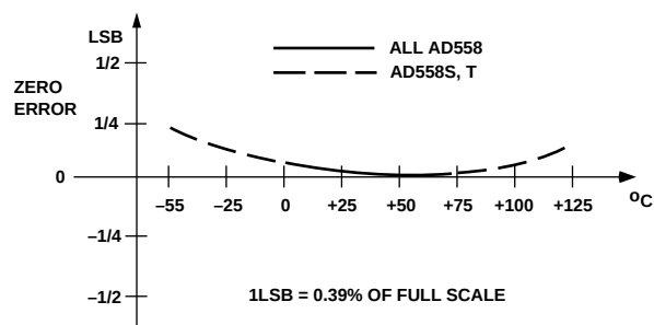
Figure 14. Zero Drift vs. Temperature Performance of AD558
