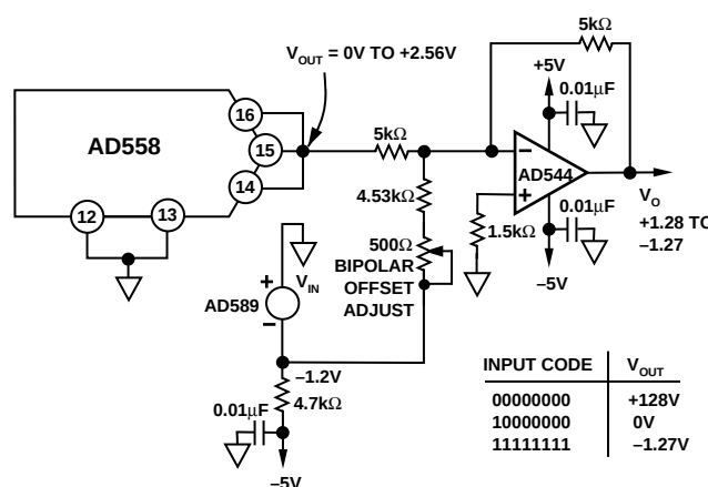
Figure 10. Bipolar Operation of AD558 from \pm 5 V Supplies
