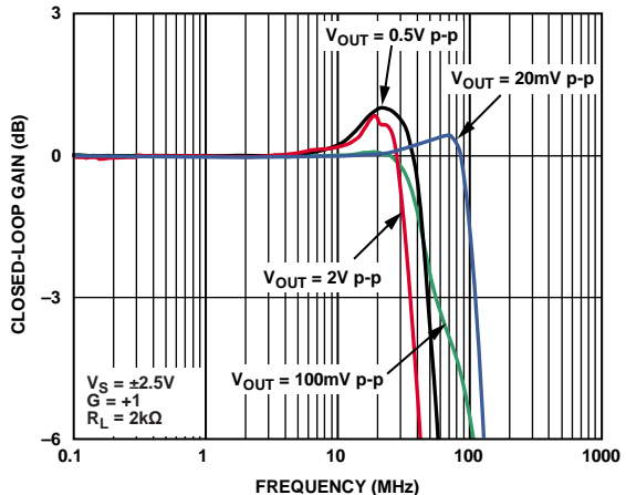
Figure 10. Frequency Response for Various Output Voltages
