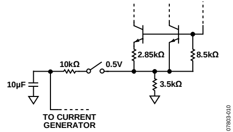
Figure 28. Equivalent VREF Circuit
