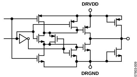
Figure 27. Equivalent Digital Output Circuit
