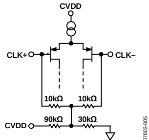
Figure 23. Equivalent Clock Input Circuit
