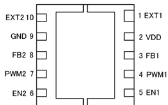
USP-10 (BOTTOM VIEW)
