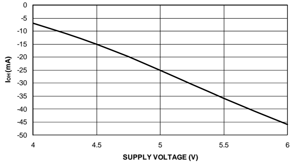
ATF750C/CL OUTPUT SOURCE CURRENT VS. SUPPLY VOLTAGE ( V_{OH} = 2.4\text{V} )
