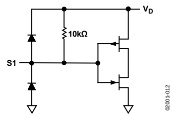
Figure 12. S1 Input
