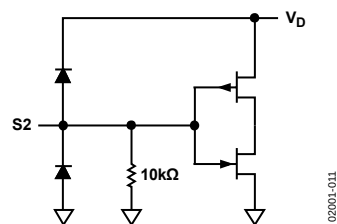
Figure 11. S2 Input
