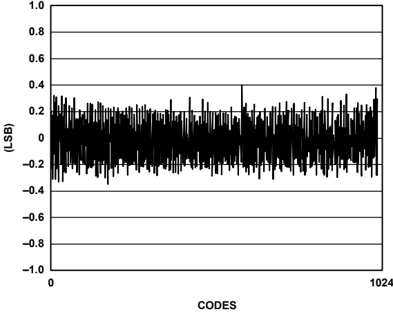
Figure 41. Typical DNL Plot, 10.3 MHz A_{IN} @ 80 MSPS
