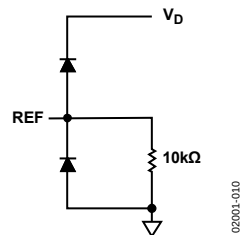
Figure 10. Reference Inputs
