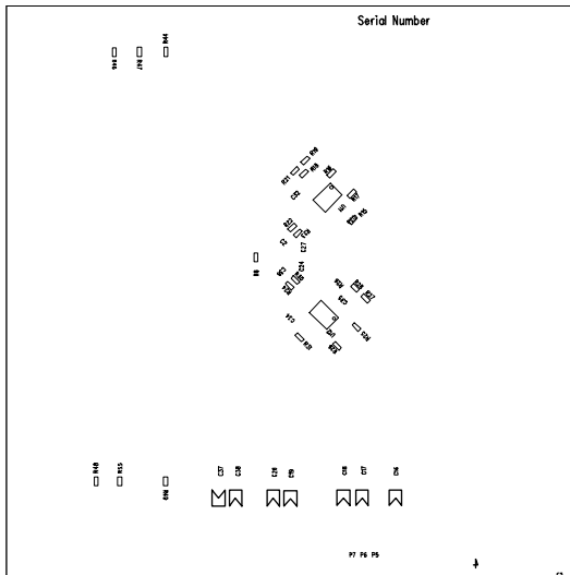
Figure 52. Bottom Silkscreen
