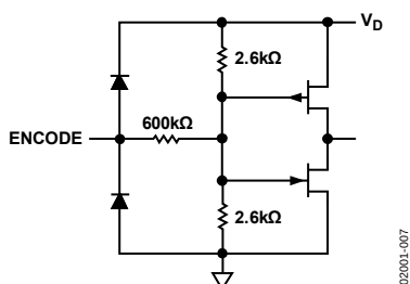
Figure 7. Encode Inputs
