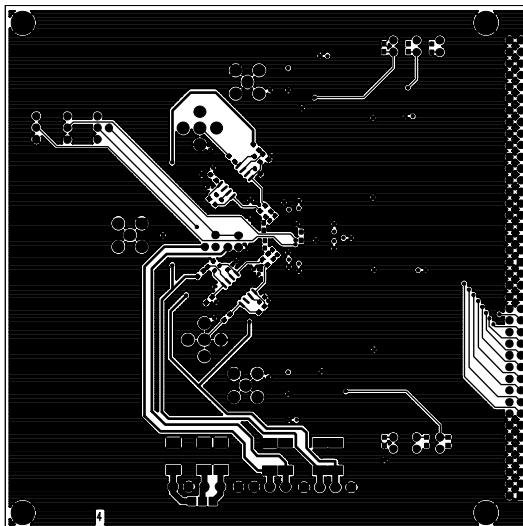
Figure 51. Bottom Routing
