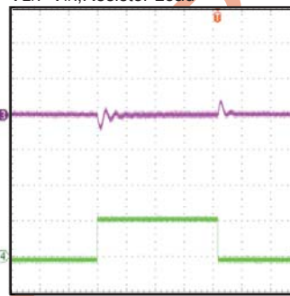
Load Transient
