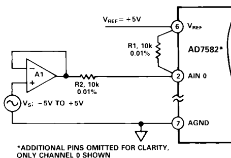
Figure 14. Bipolar -5V to +5V Operation
