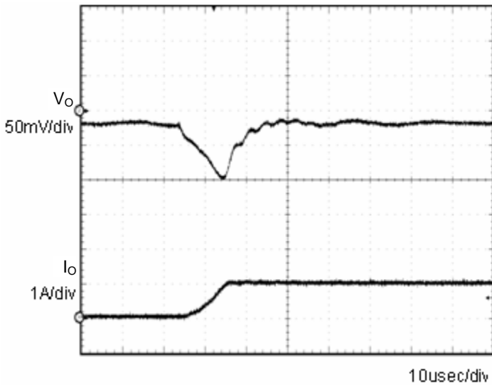
Fig.3 Transient Response (0→1.0A) Co=1µF
