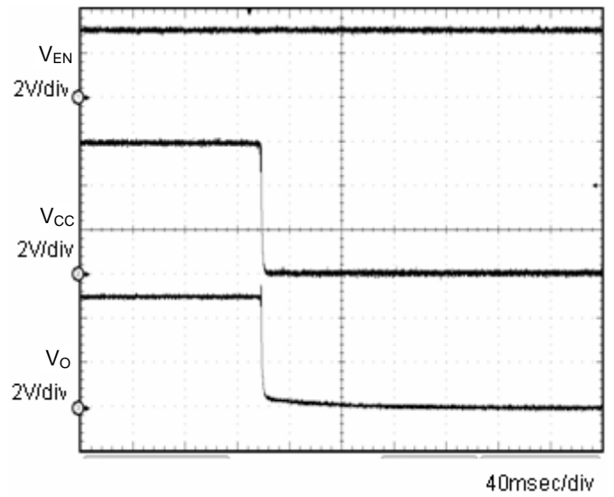
Fig.6 OFF sequence 1 Co=1µF
