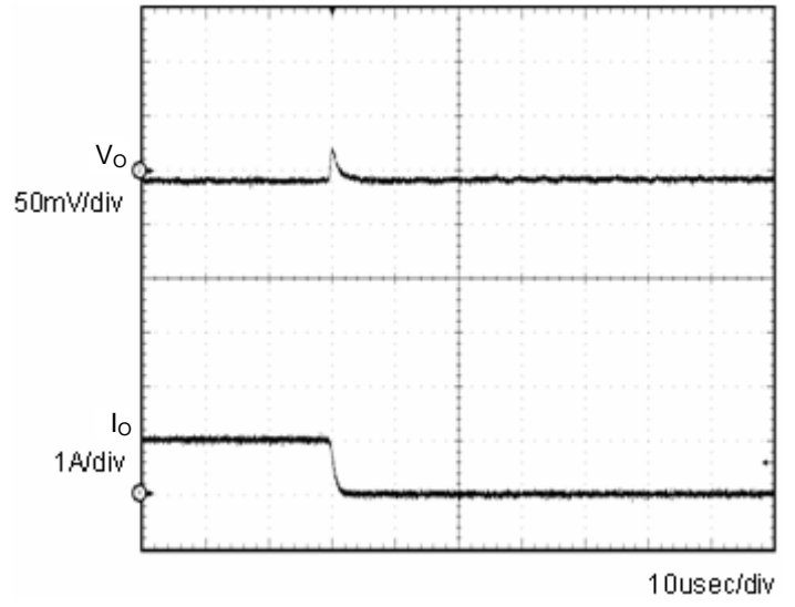
Fig.4 Transient Response (1.0→0A) Co=1µF
