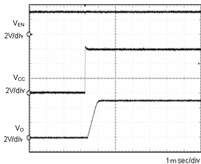
Fig.5 Input sequence 1 \text{Co}=1\mu\text{F}
