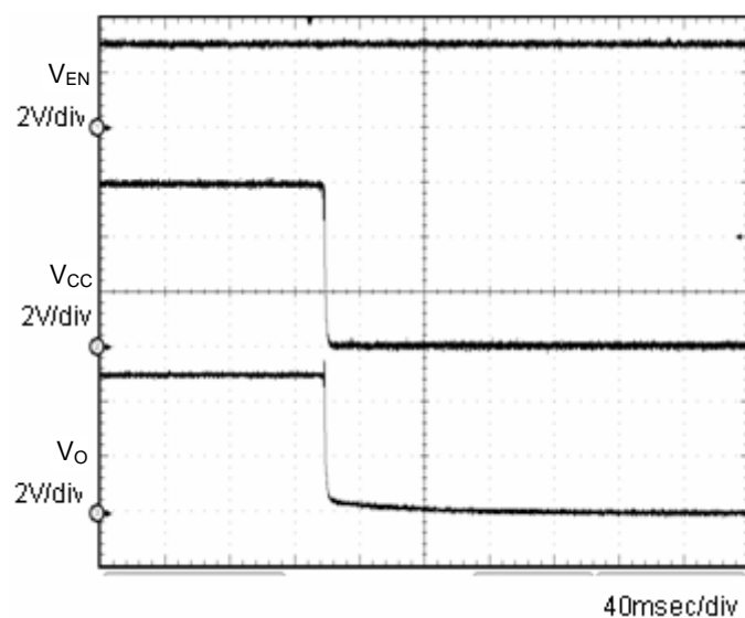
Fig.6 OFF sequence 1 \text{Co}=1\mu\text{F}
