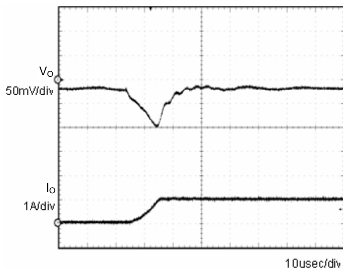
Fig.3 Transient Response (0→1.0A) \text{Co}=1\mu\text{F}
