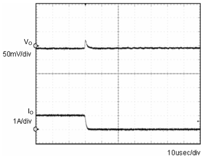
Fig.4 Transient Response (1.0→0A) \text{Co}=1\mu\text{F}
