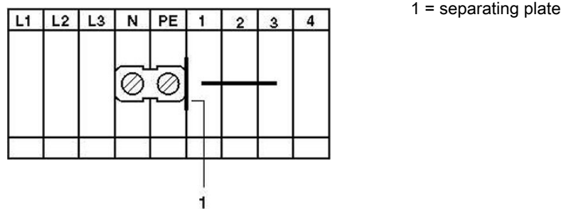
Circuit diagram
