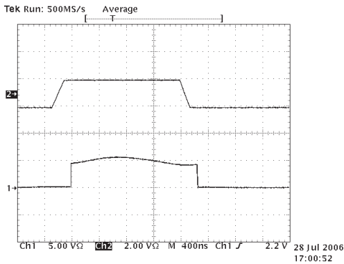
Receiver Propagation Delay (SP3083E-SP3085E)
