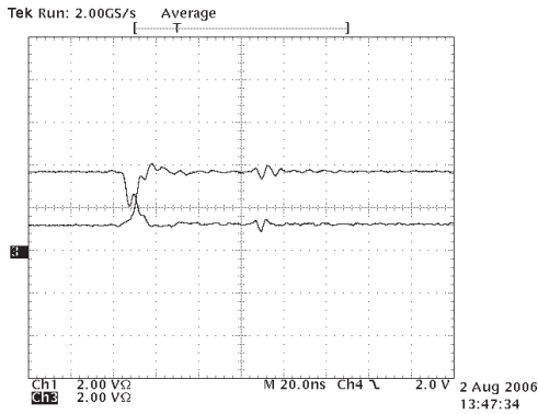
Driver Output Waveforms High to Low (SP3086E-SP3088E)
