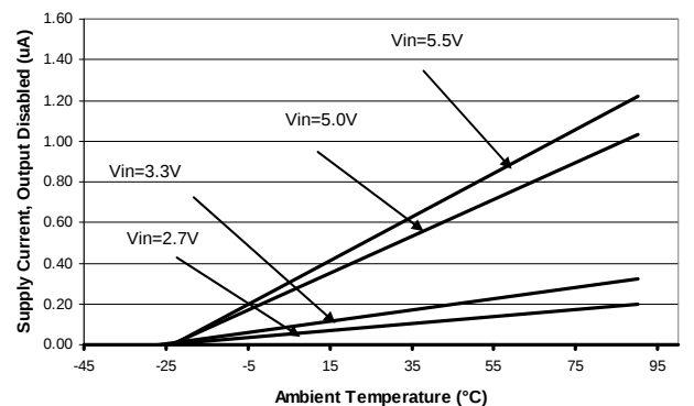
Supply Current, Output Disabled vs Ambient Temperature
